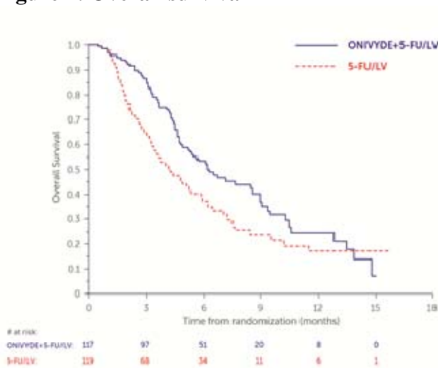
Figure 1: Overall survival
