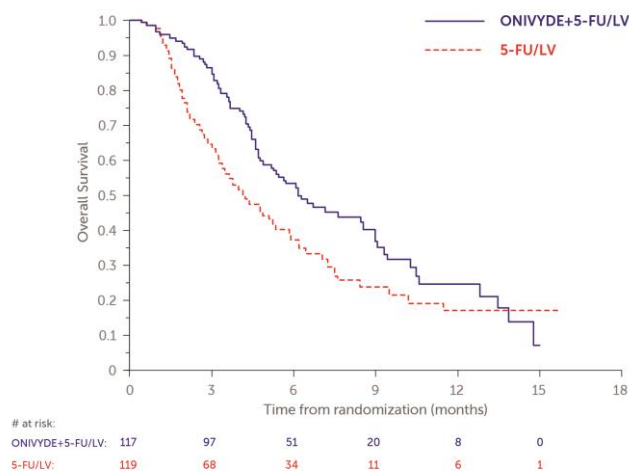
Figure 1: Overall survival
